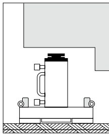
1. Stage: Initial position, stage lift rests on the ground under the load.
