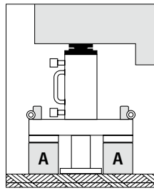
3. Stage: Two support bars type „A“ are positioned in place.
