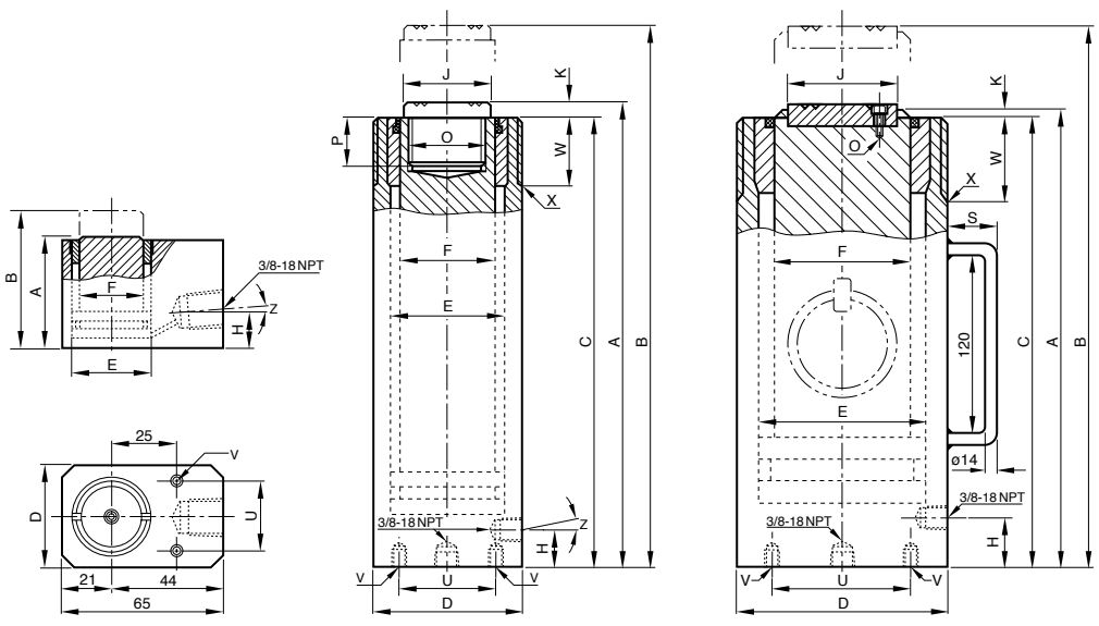
Model YS-5/15
