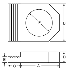
Lifting claws
