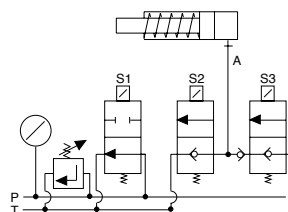
VEP-3/3-1 and VEP-3/3-2 for single-acting cylinders
