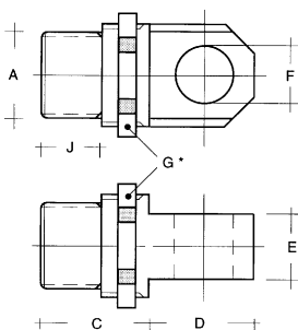
AYS-...-1 for cylinder base
