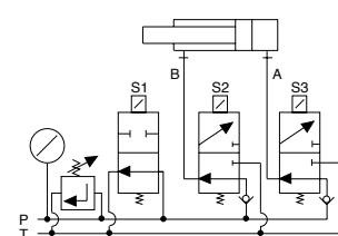
VEP-4/3-1 and VEP-4/3-2 for double-acting cylinders
