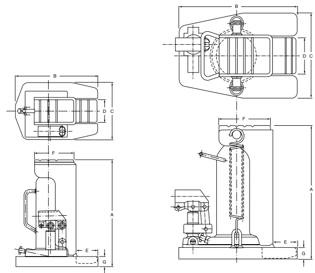
Model YAM 2
