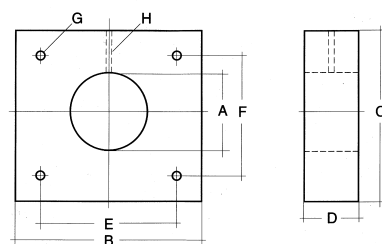
Model AYP
