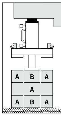
9. Stage: Piston is retracted, middle bar type „B“ is inserted and lifts the 4th step on middle bar „B“ and so on...
