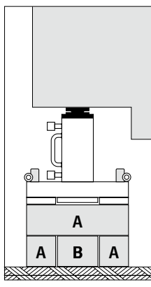
7. Stage: Two bars „A“ are inserted and rotated at 90°, piston is retracted and middle bar is inserted.
