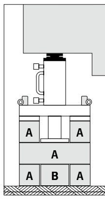
8. Stage: Load is lifted on middle bar (3rd step), two support bars type „A“ are positioned at 90° and load rests on support bars „A“.
