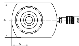
Model YFS
