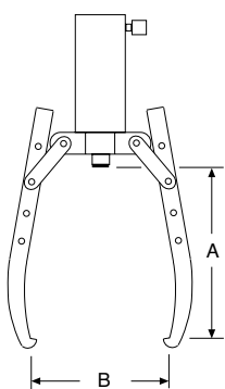
Models BMZ-1010 and BMZ-1510
